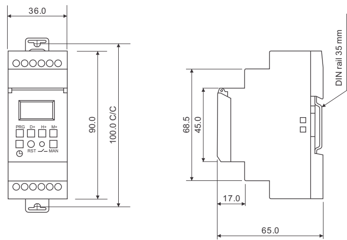
Overall Dimensions
