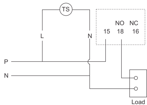
Connection Diagrams
